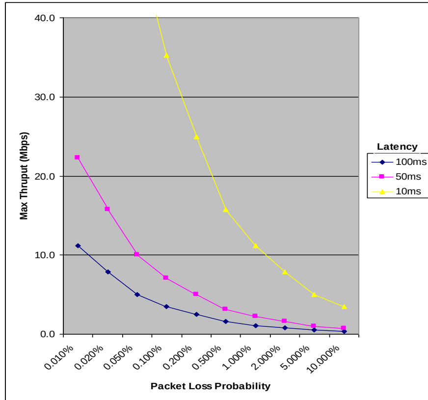
Figure 8.5: Impact of Packet Loss on Throughput
